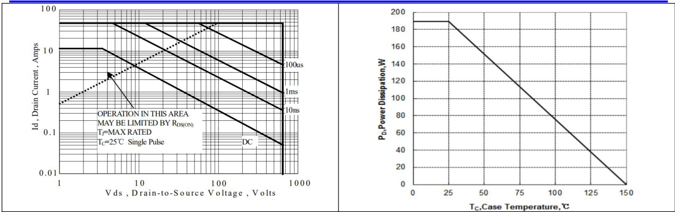
Maximum Forward Bias Safe Operating Area
