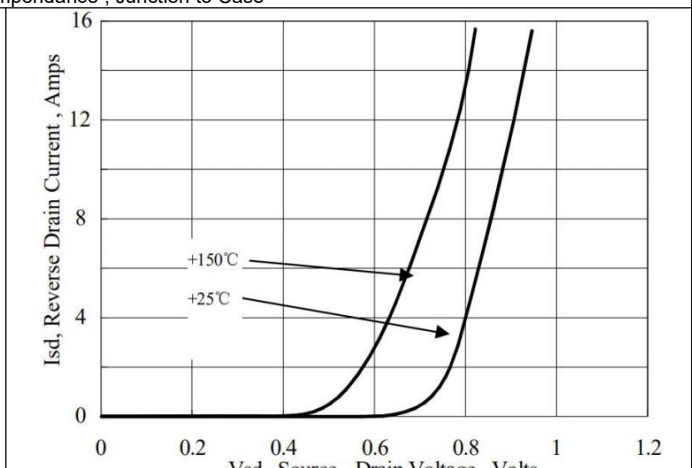
Typical Body Diode Transfer Characteristics
