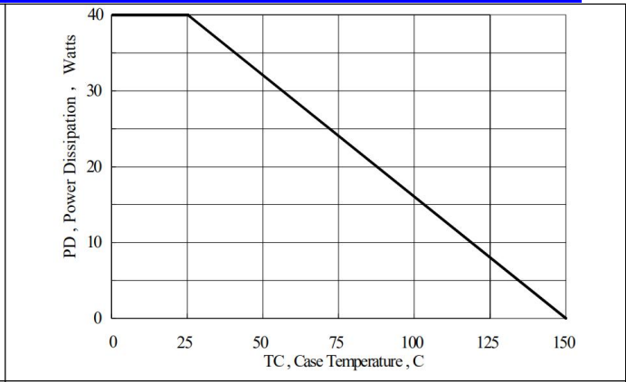
Maximum Power Dissipation vs Case Temperature
