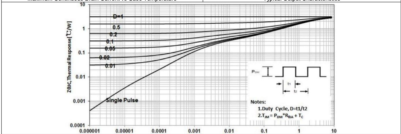
Maximum Effective Thermal Impedance, Junction to Case
