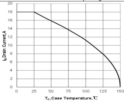
Maximum Continuous Drain Current vs Case Temperature
