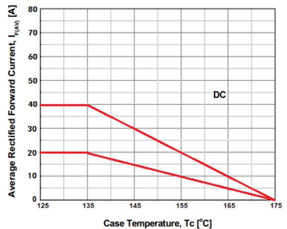
FIGURE 4. CURRENT DERATING CURVE
