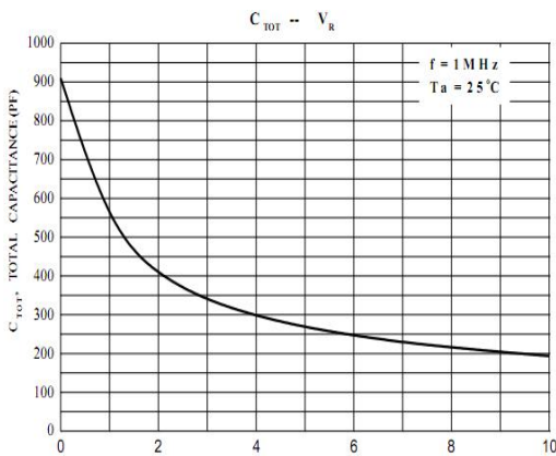
FIGURE 1. Total capacitance vs Voltage
