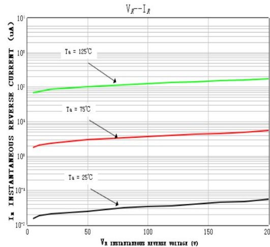
FIGURE 2. REVERSE CURRENT vs REVERSE VOLTAGE
