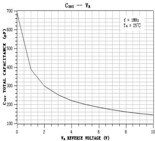
FIGURE 1. Total capacitance vs Voltage
