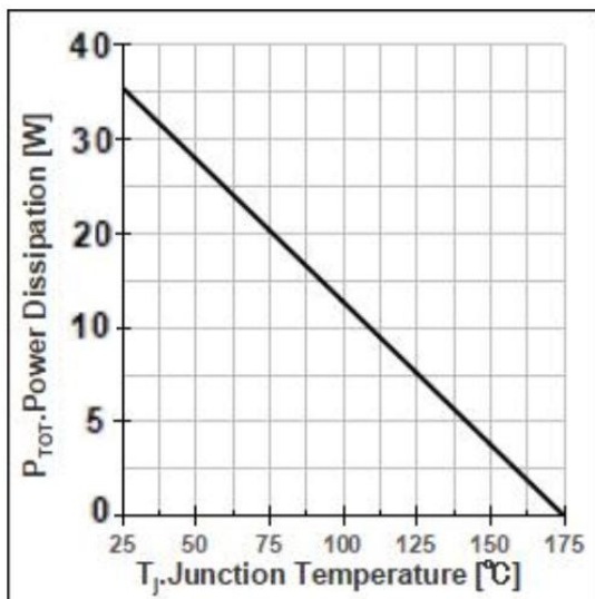
Fig15. Power dissipation temperature characteristic
