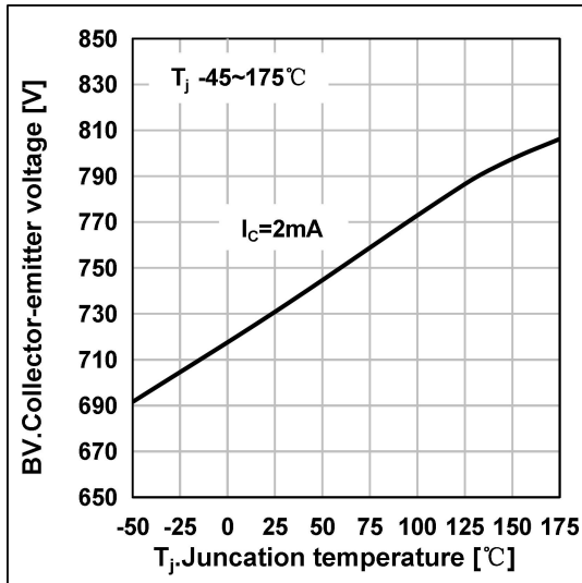
Fig1. Collector-Emitter Breakdown Voltage Temperature characteristic
