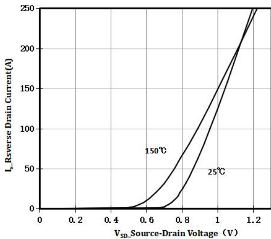
Fig 9 Source- Drain Diode Forward
