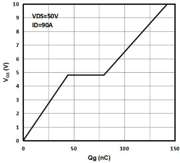
Fig 7 Gate Charge Figure
