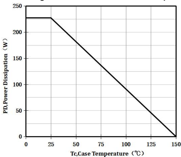
Fig 5 Power De-rating
