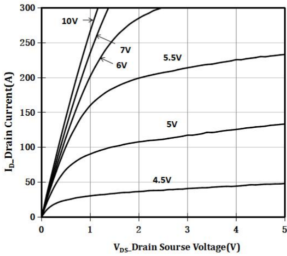
Fig 1 Output Characteristics
