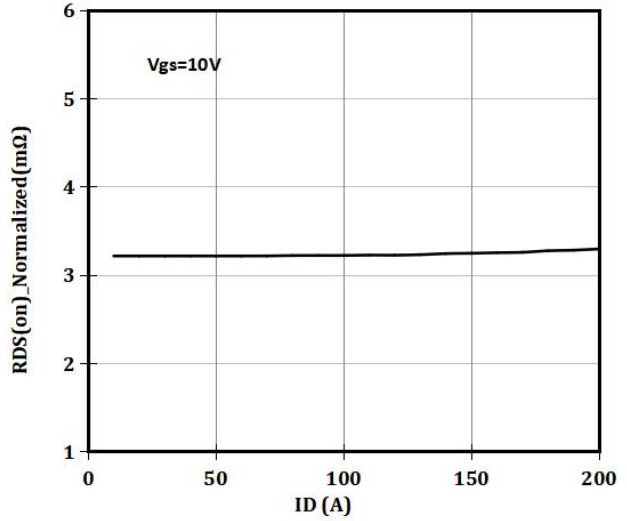
Fig 8 RDSON vs Drain Current
