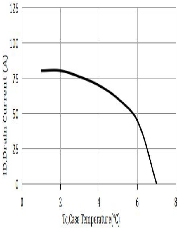
Figure 6. Power De-rating
