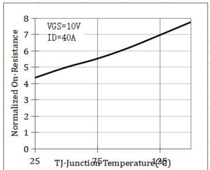
Figure 4. Rdson vs Temperature
