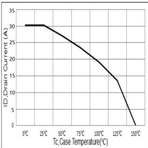
Figure 7. ID Current De-rating
