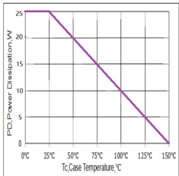
Figure 8. Power De-rating
