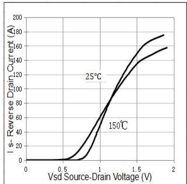
Figure 4. Source-Drain Diode Forward
