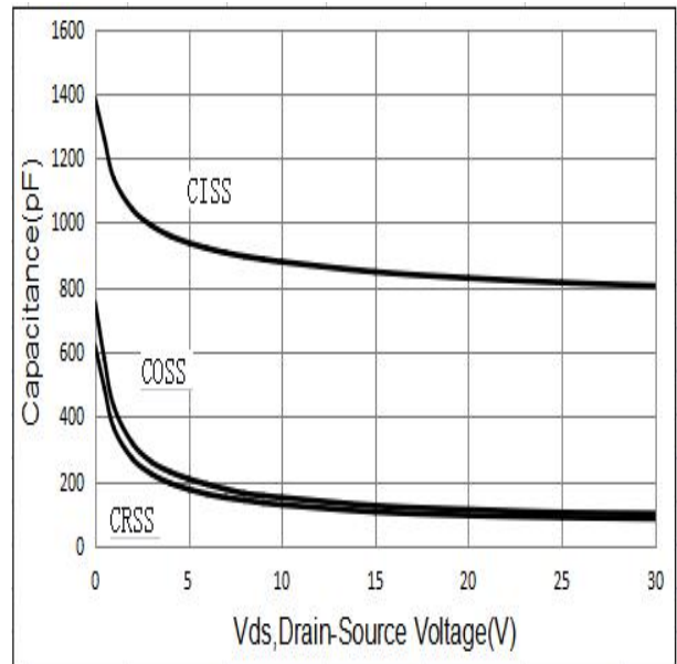
Figure 6. Capacitance Characteristics
