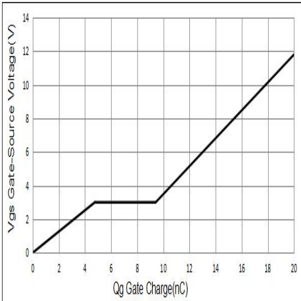
Figure 5. Gate Charge Characteristics
