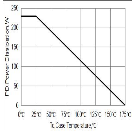
Figure 9. Power De-rating
