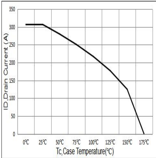
Figure 8. ID Current De-rating
