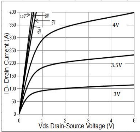
Figure 1 Output Characteristics
