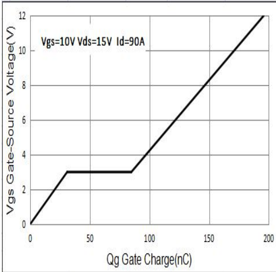
Figure 4. Gate Charge
