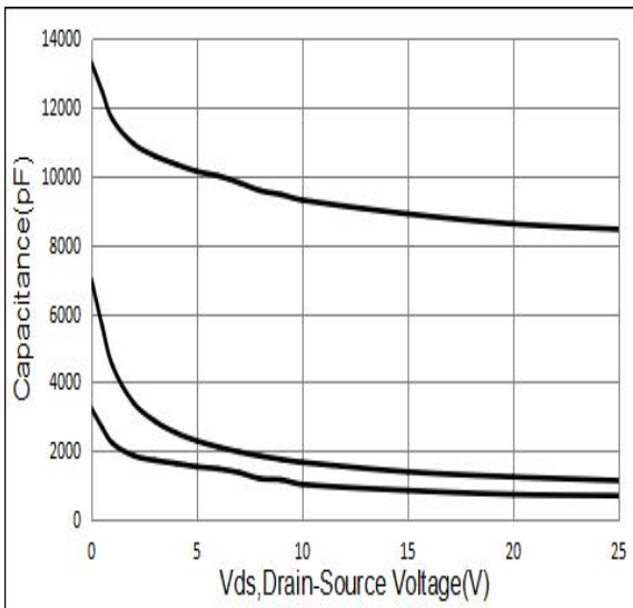
Figure 6. Capacitance Characteristics
