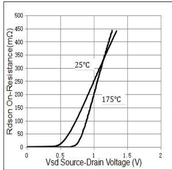
Figure 5. Source-Drain Diode Forward
