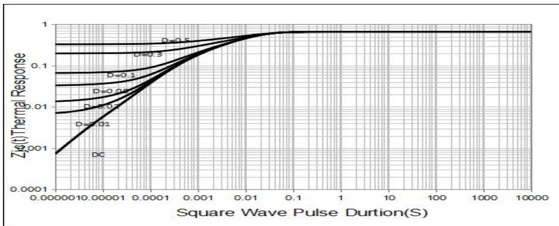
Fig 10. Normalized Maximum Transient Thermal Impedance
