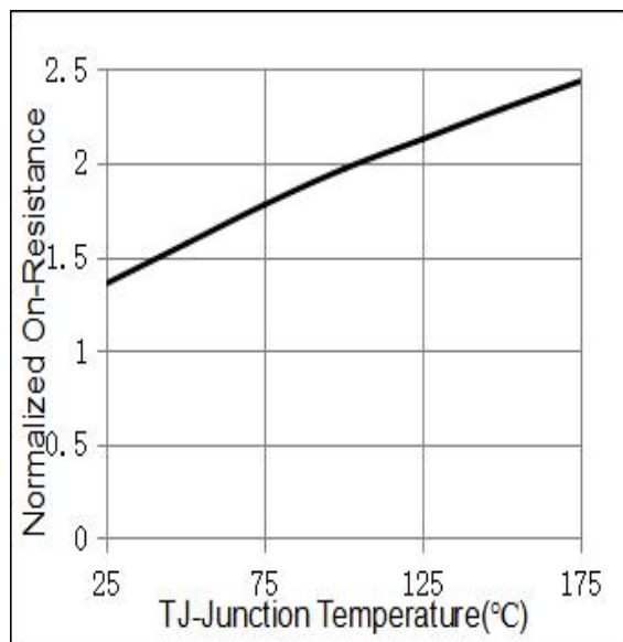
Figure 3. Rdson vs Temperature
