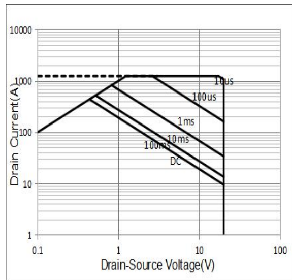
Figure 7. Safe Operation Area
