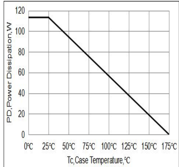
Figure 9. Power De-rating
