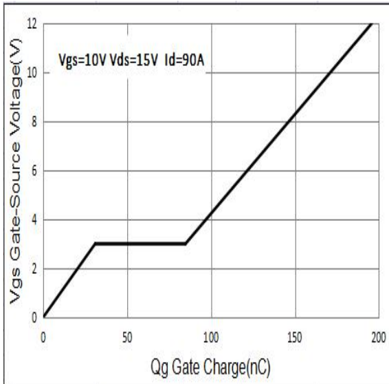
Figure 4. Gate Charge
