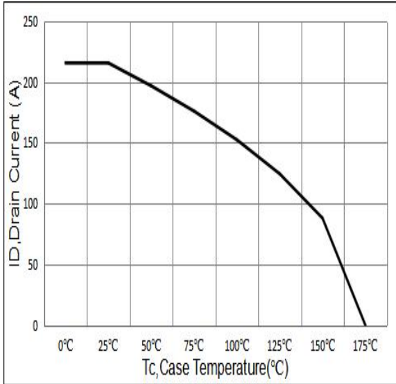
Figure 8. ID Current De-rating
