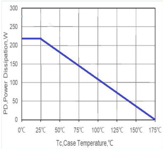
Figure 5. Power De-rating
