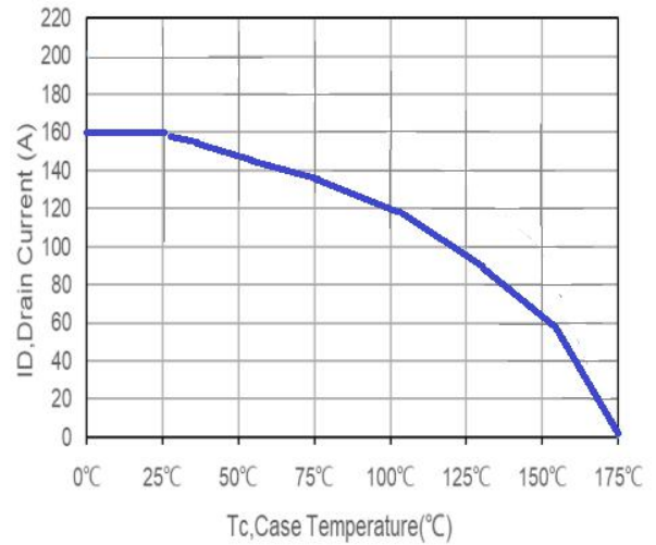
Figure 6. ID Current Derating
