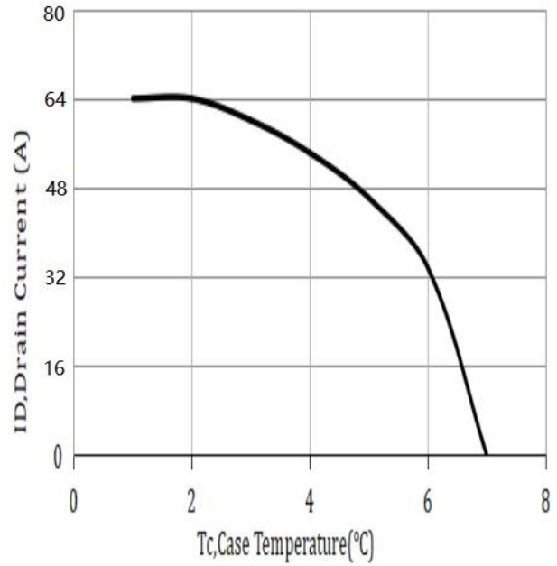
Figure 6. ID Current Derating
