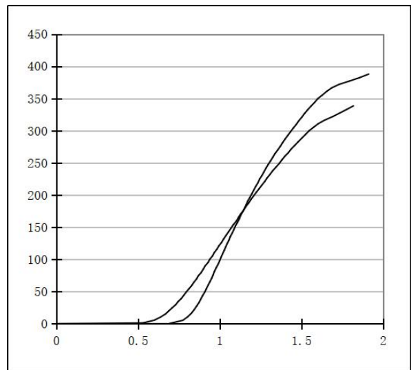
Fig 4. Source-Drain Diode Forward
