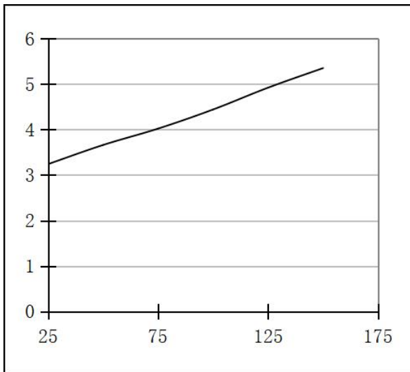
Figure 3. Rdson vs Temperature
