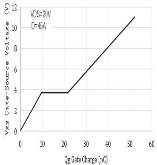
Figure 8. Gate Charge Characteristics
