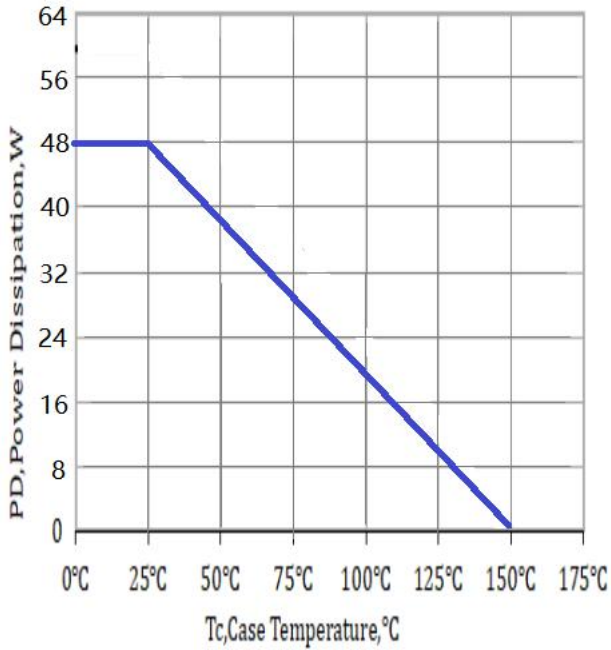
Figure 5. Power De-rating
