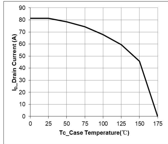
Figure 8 Current De-rating
