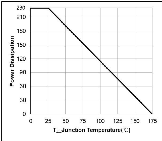
Figure 7 Power De-rating
