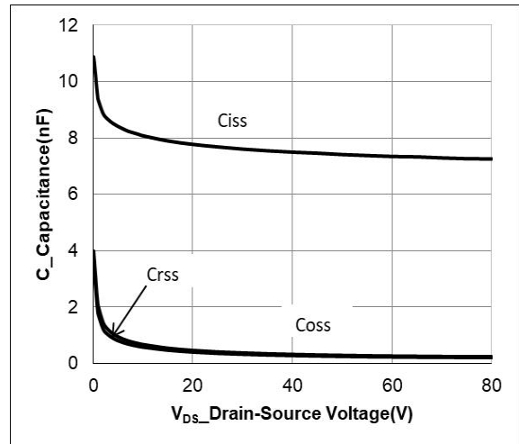
Figure 4 Capacitance Vs V_{DS}
