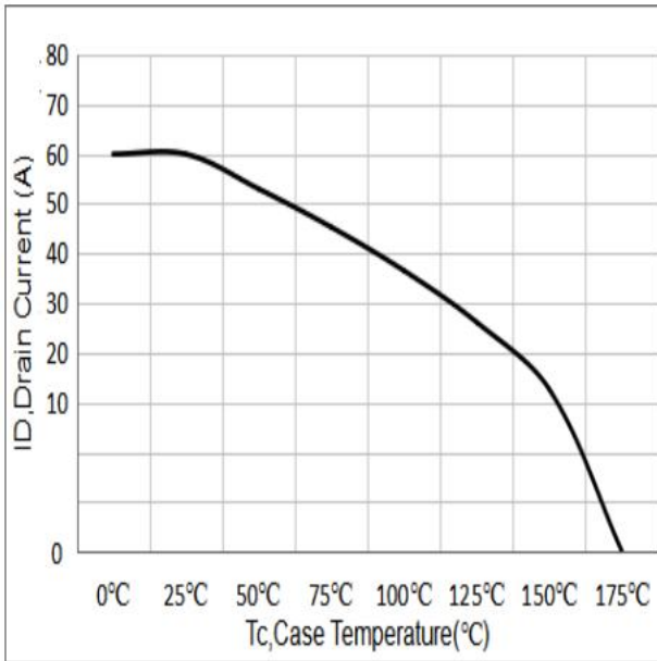
Figure 5. ID Current Deratin
