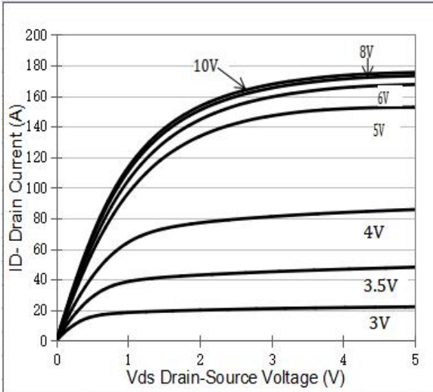
Figure 1 Output Characteristics
