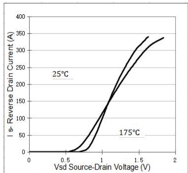
Fig 4. Source-Drain Diode Forward
