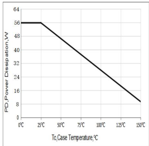
Figure 6. Power De-rating
