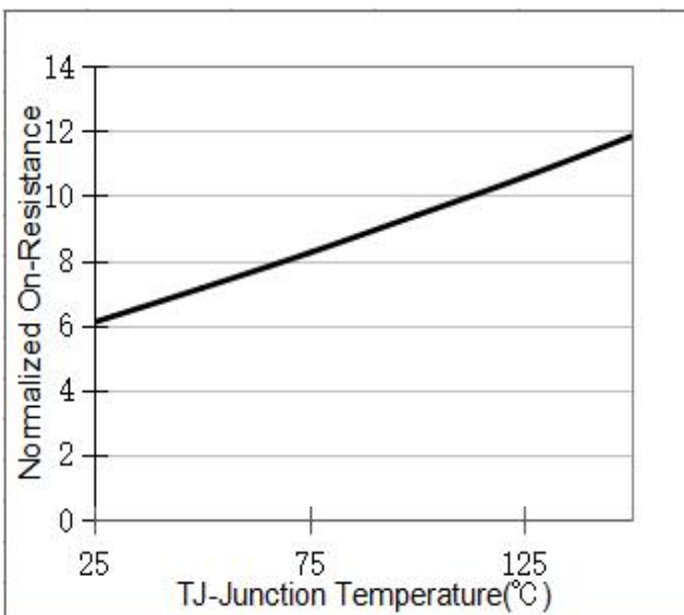
Figure 3. Rdson vs Temperature
