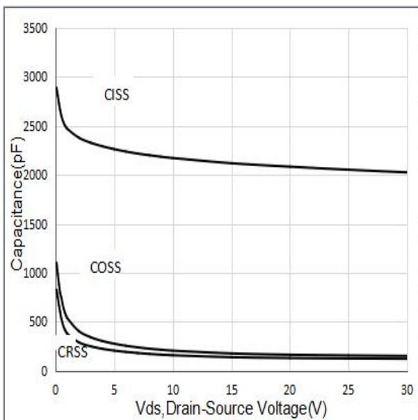
Figure 7. Capacitance Characteristics
