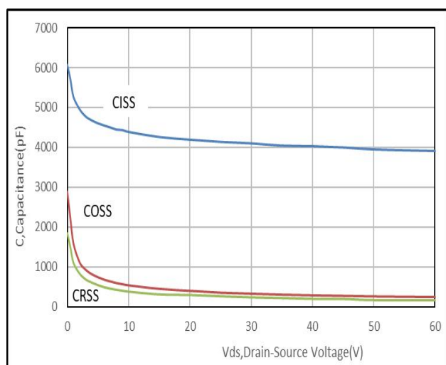
Fig 7 Capacitances vs Vds
