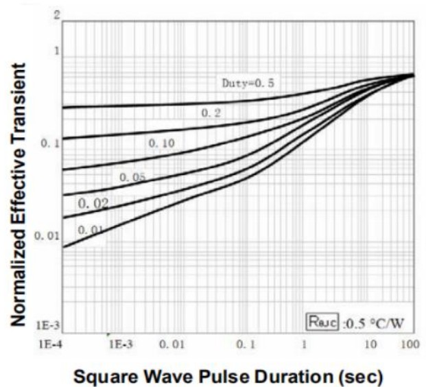
Fig 12. Thermal Transient Impedance
