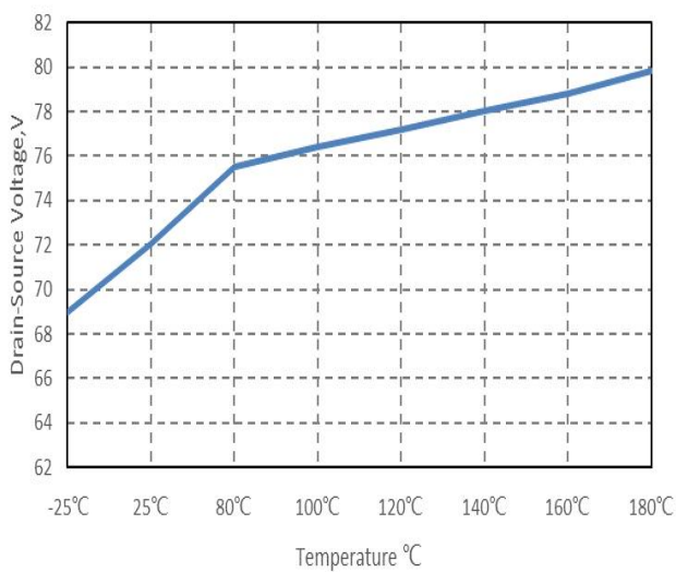
Fig 3 BVDSS vs Junction Temperature
