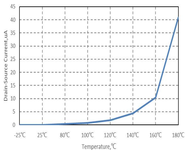
Fig 6 IDSS vs Junction Temperature
