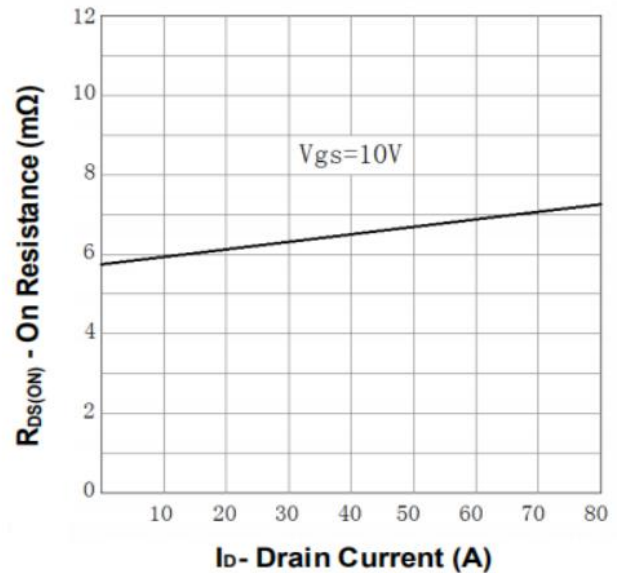
Fig 10. Drain-Source On Resistance
