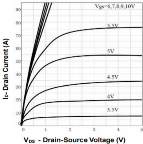
Fig 1. Output Characteristics
