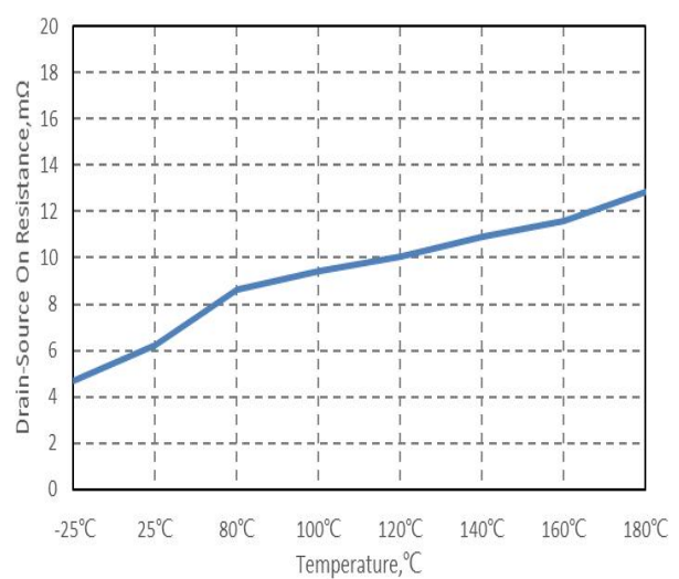
Fig 4 RDS(on) vs Junction Temperature
