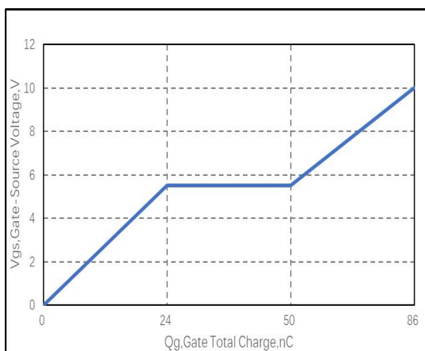
Fig 8 Gate Charge
