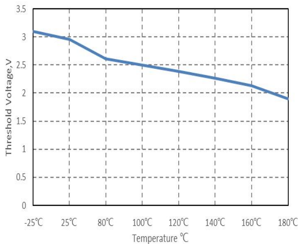
Fig 5 VTH vs Junction Temperature
