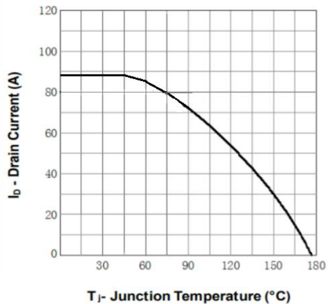
Fig 2. Drain Current
