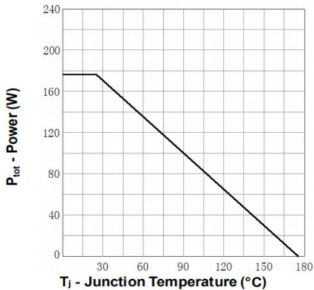
Fig 9. Power Dissipation
