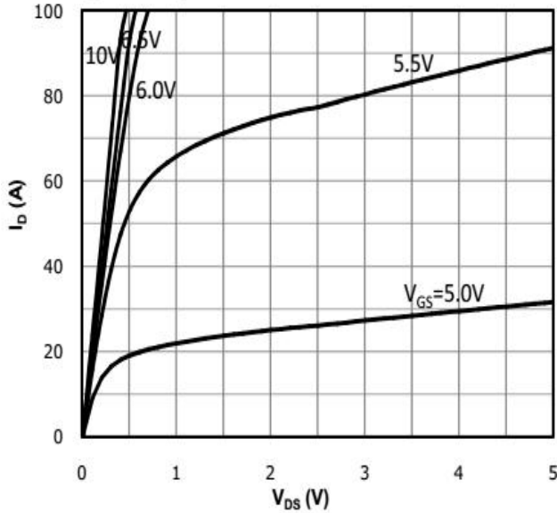
Fig 1: Output Characteristics
