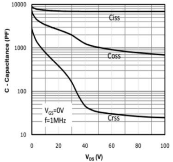
Fig 6: Capacitance Characteristics
