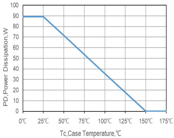
Figure 5. Power De-rating
