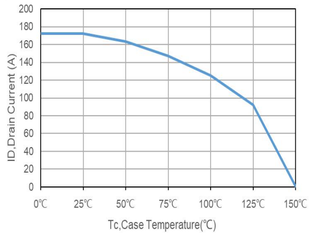
Figure 6. ID Current Derating
