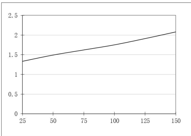
Figure 3. Rdson vs Temperature
