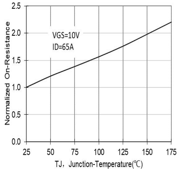
Fig 4. Rdson-Junction Temperature
