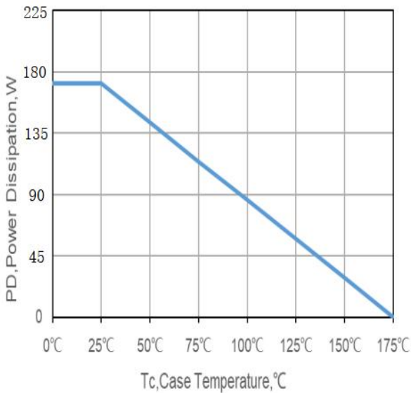
Fig 8. Power De-rating
