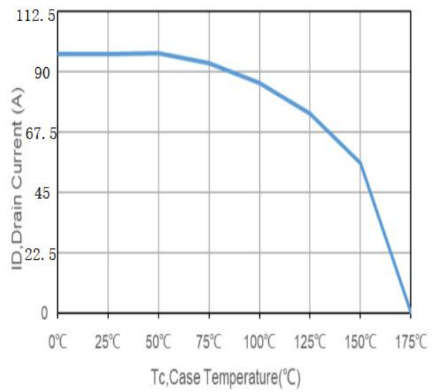
Fig 9. Current De-rating
