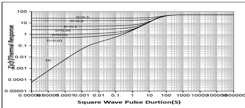
Fig 11. Normalized Maximum Transient Thermal Impedance
