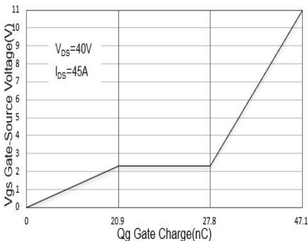
Fig 5. Gate Charge
