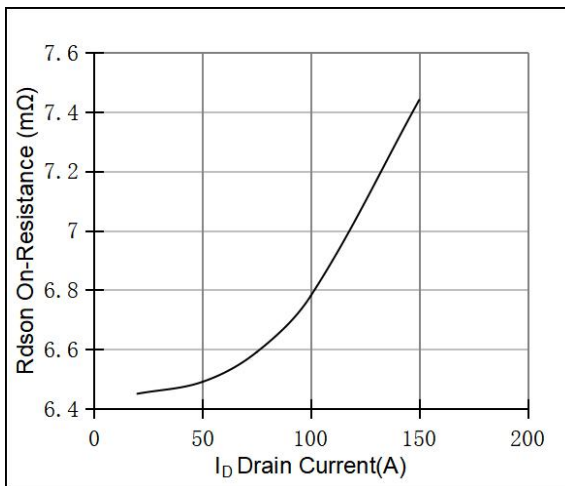
Fig 3. Rdson-Drain Current
