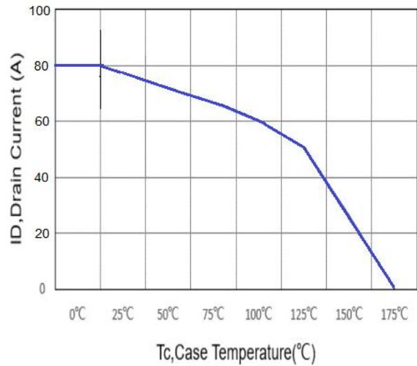
Fig 10. Current De-rating
