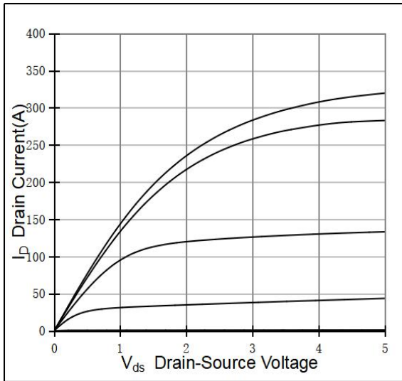
Fig 1. Output Characteristics
