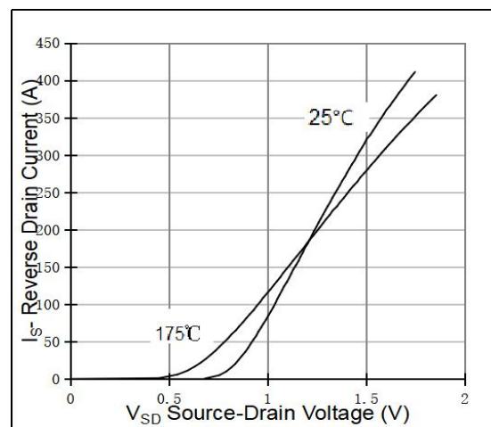
Fig 6. Source-Drain Diode Forward
