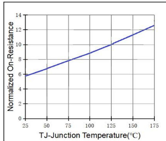
Fig 4. Rdson-Junction Temperature
