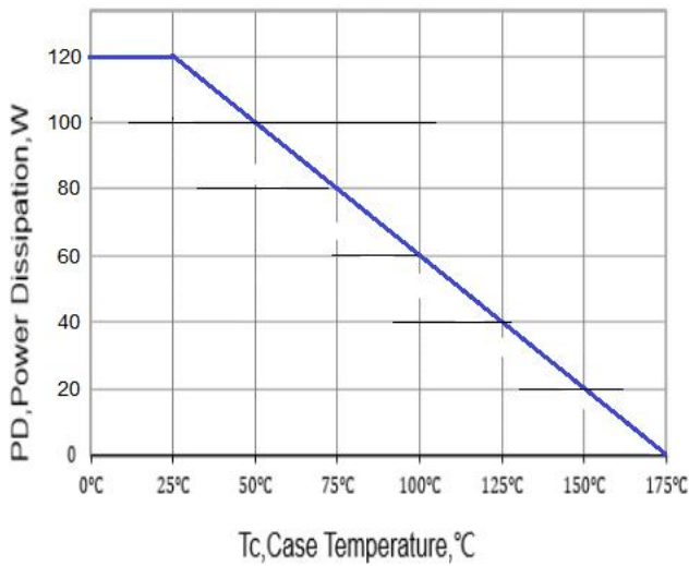
Fig 9. Power De-rating
