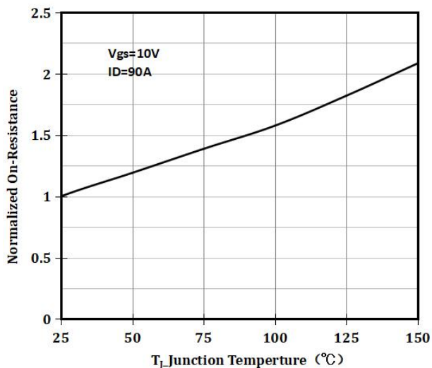
Figure 3. Rdson vs Temperature
