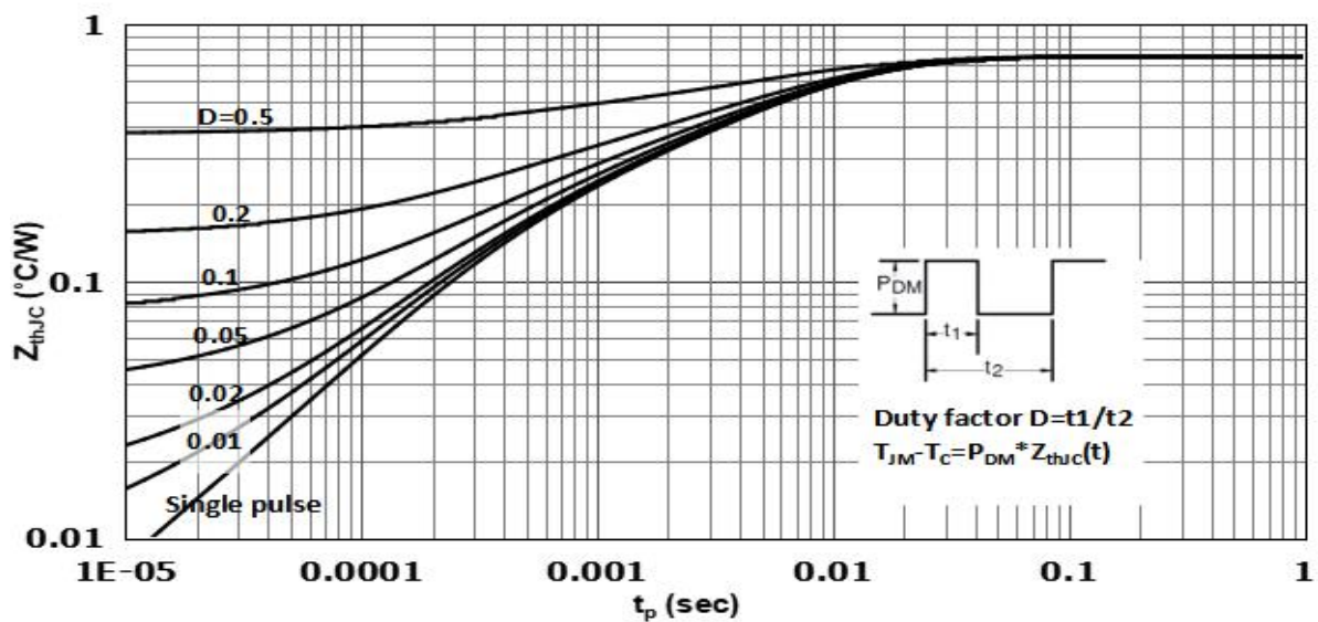
Figure 10. Max. Transient Thermal Impedance
