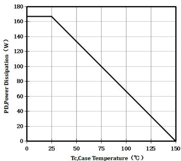
Figure 5. Power De-rating
