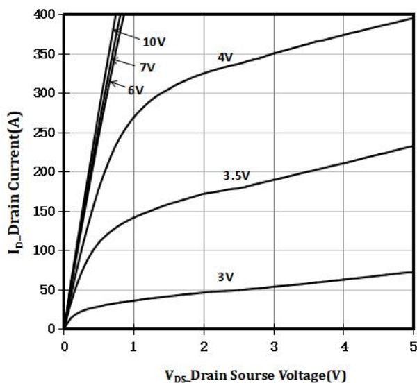
Figure 1 Output Characteristics
