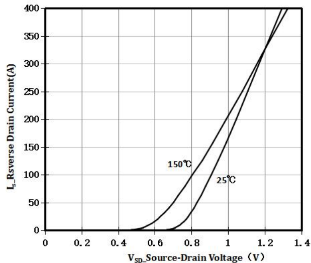
Figure 4. VSD_ Source-Drain Diode forward
