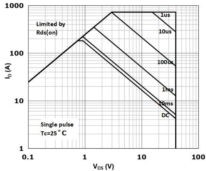
Figure 9. Safe Operating Area
