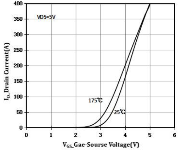
Fig 2. Transfer Characteristics
