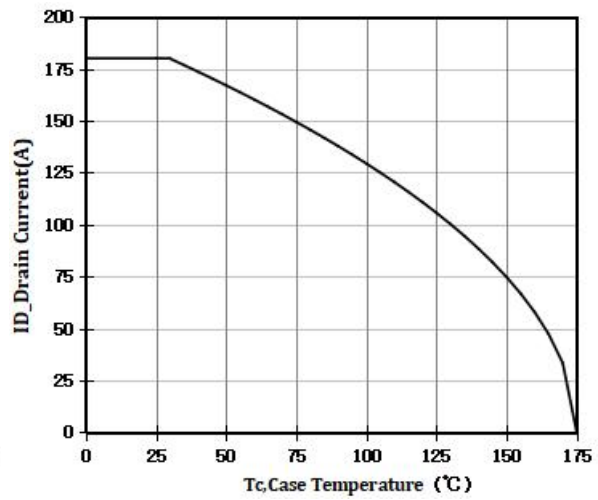
Fig 8. Current De-rating
