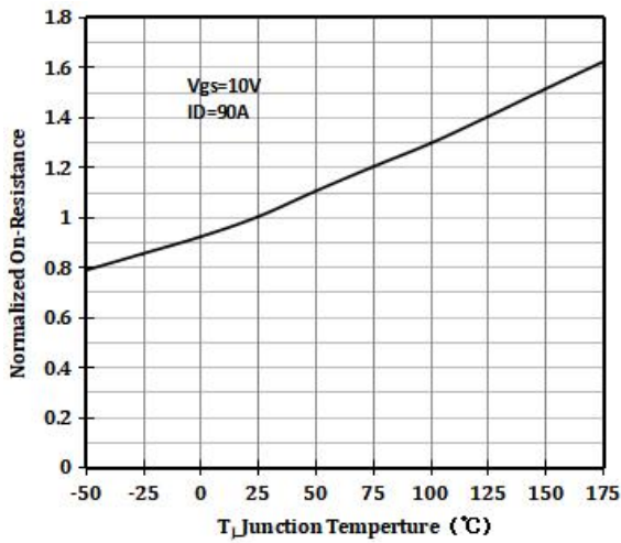
Fig 3. Rdson-Junction Temperature
