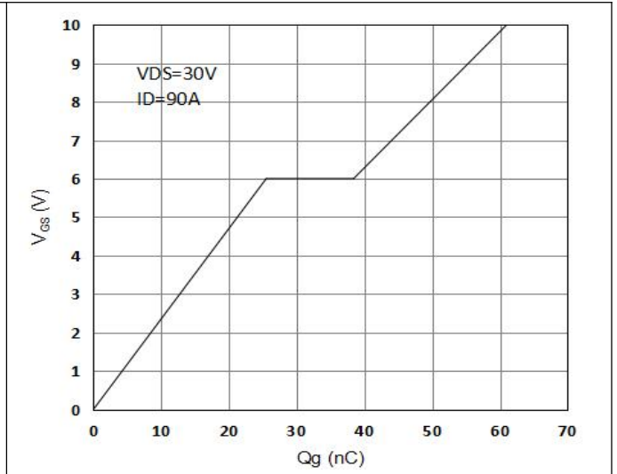
Figure 4 Gate Charge
