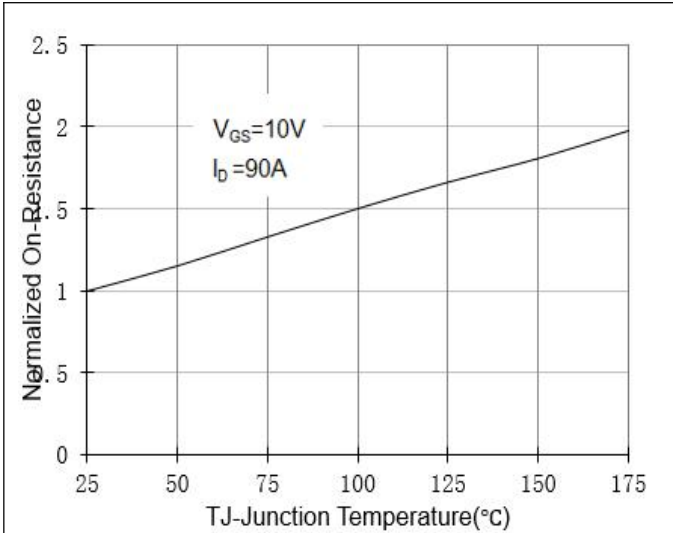
Figure 3 Rds(on)-Junction Temperature
