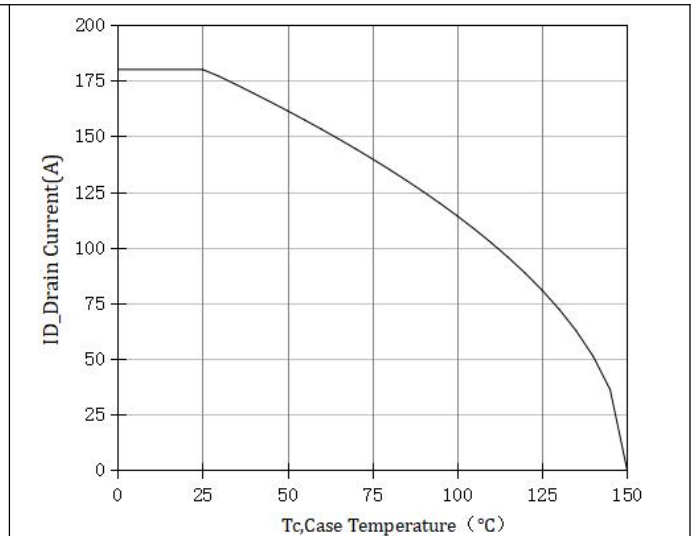
Figure 8 Current De-rating
