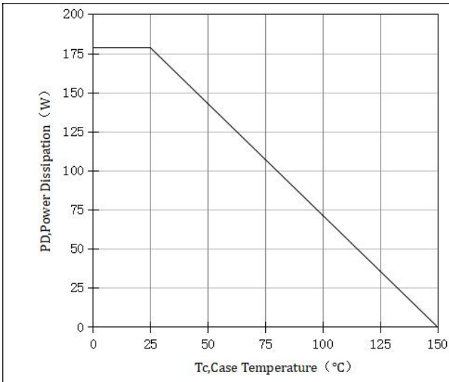
Figure 7 Power De-rating
