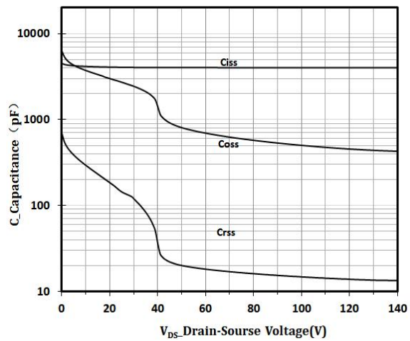
Fig 4 Capacitance vs Vds
