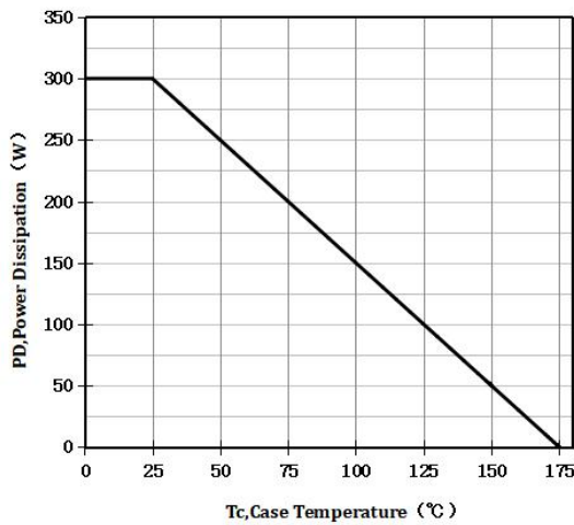
Fig 5 Power De-rating
