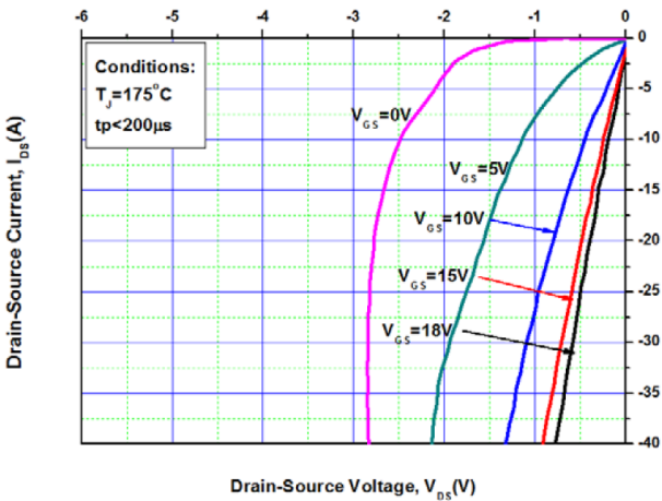
Figure 11. 3rd Quadrant Characteristic at 175°C
