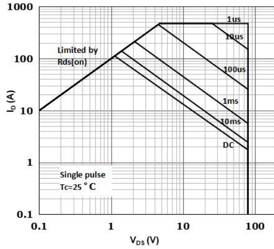
Figure 8. Safe Operating Area
