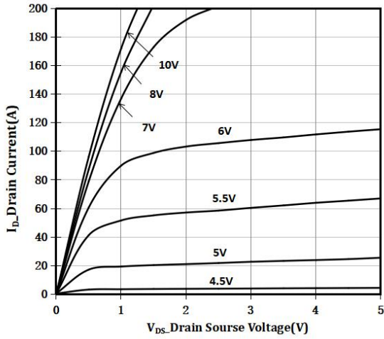
Fig 1. Output Characteristics
