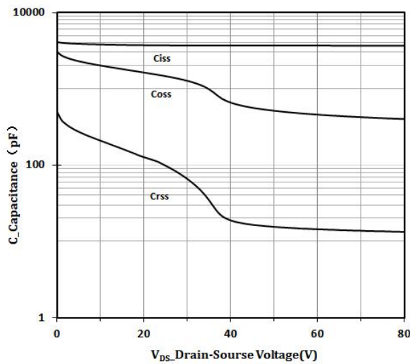
Figure 9. Capacitance Characteristics
