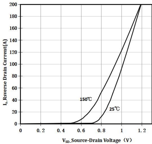
Figure 3 Source-Drain Diode Forward
