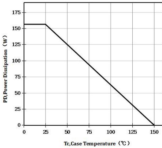
Figure 7. Power Dissipation
