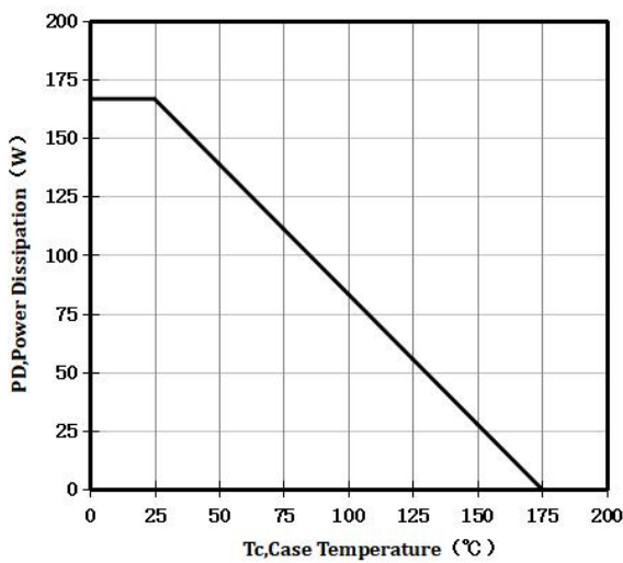
Figure 5 Power De-rating
