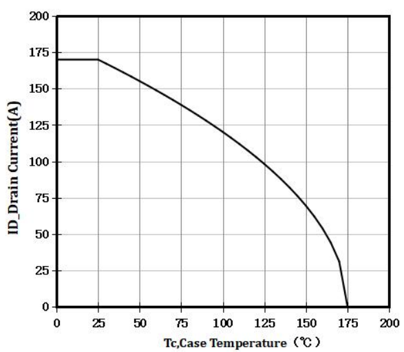
Figure 6 Current De-rating
